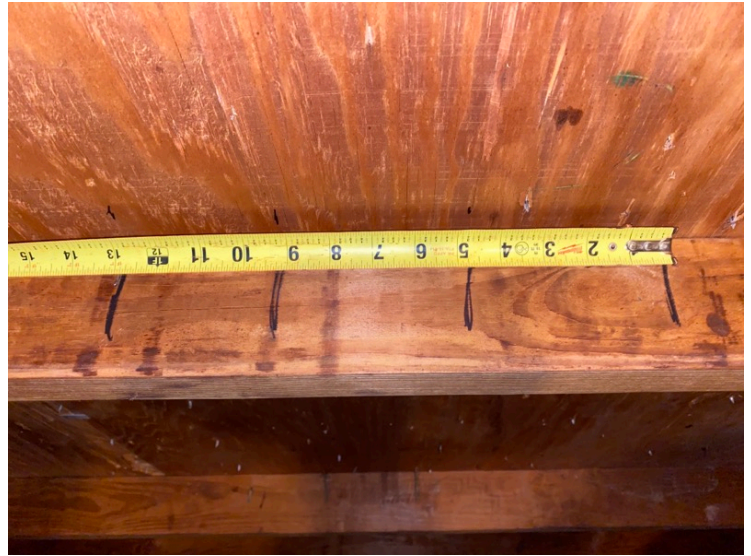
Nail Spacing
